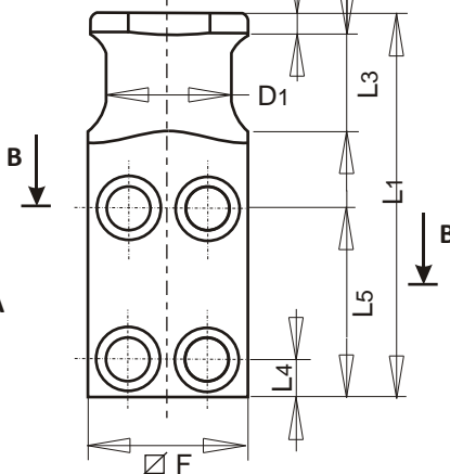
FORMA “B” FORM “B”
