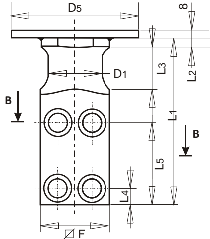
FORMA “B” FORM “B”
